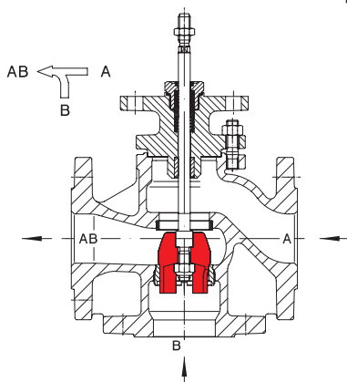
Design with mixing plug DN 15-150
