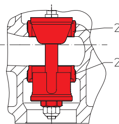
Mixing plug with two screwed seat rings (standard at DN125/150 and design with stainless steel)
