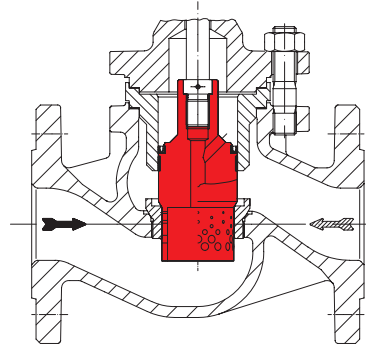
Perforated pressure balanced plug
