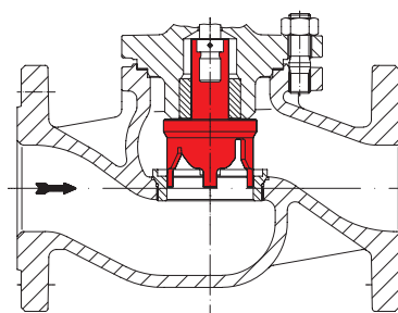
V-port plug with post and port guiding
