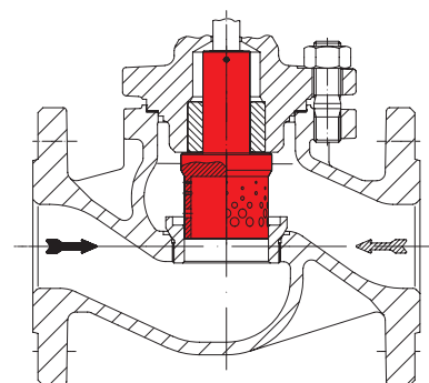
Perforated plug with post and port guiding
